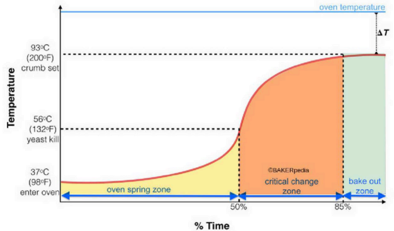
Figure 4. A thermal profiling curve
